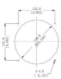
OUTLET SIDE
