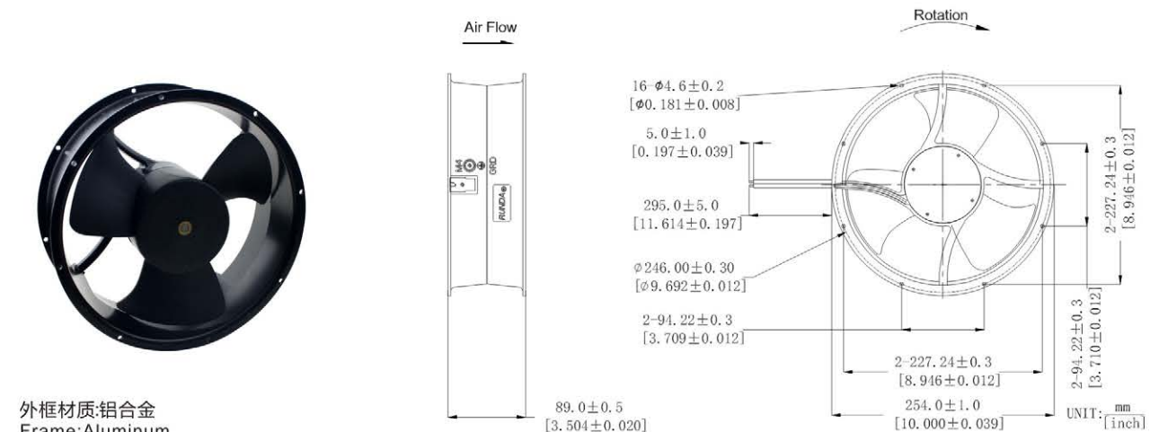
DIMENSIONS DRAWING
