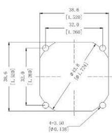
INLET SIDE
