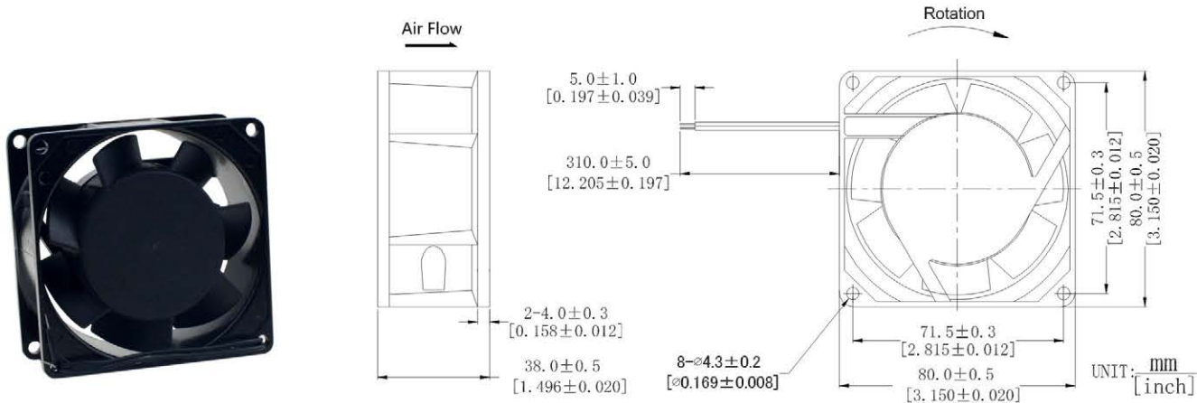
DIMENSIONS DRAWING
