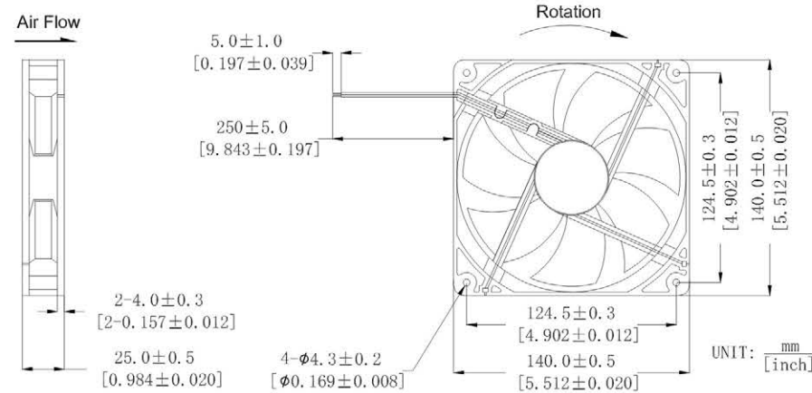
DIMENSIONS DRAWING
