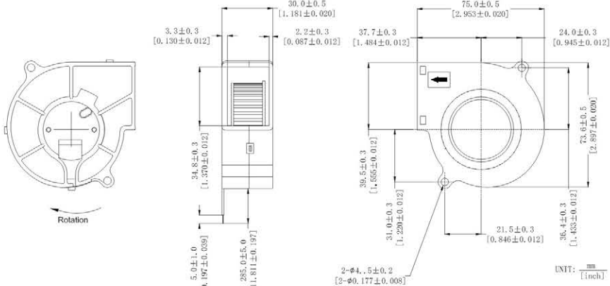
DIMENSIONS DRAWING
