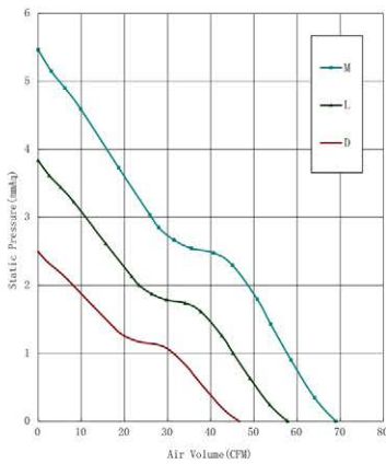
Fan Performance Curve
