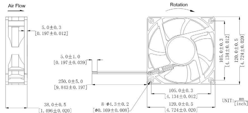
DIMENSIONS DRAWING
