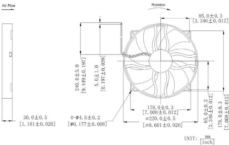
DIMENSIONS DRAWING
