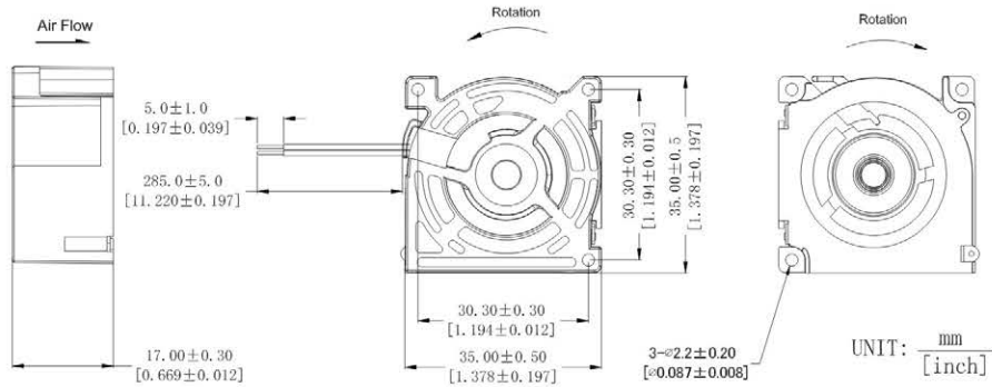
DIMENSIONS DRAWING
