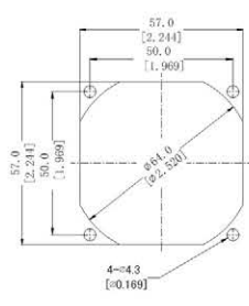
OUTLET SIDE
