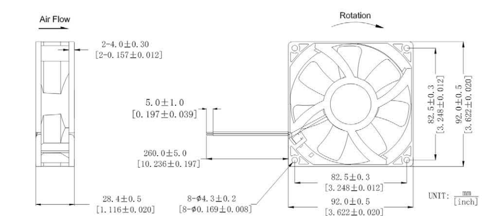
DIMENSIONS DRAWING
