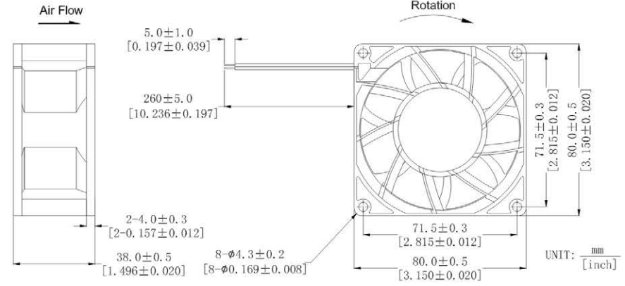
DIMENSIONS DRAWING
