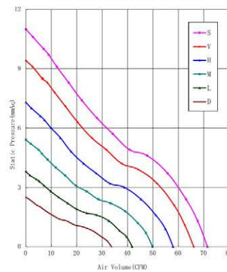
Fan Performance Curve
