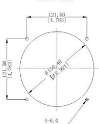
INLET SIDE
