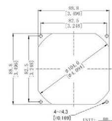
INLET SIDE
