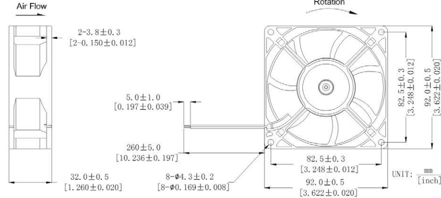
DIMENSIONS DRAWING
