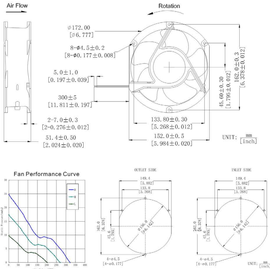
DIMENSIONS DRAWING
