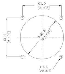
INLET SIDE
