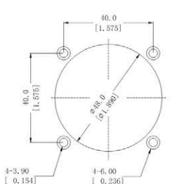
INLET SIDE
