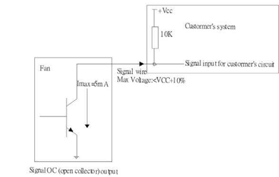
PWM输入标准接口电路/PWM input standard circuit diagram
