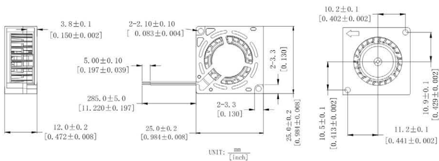
DIMENSIONS DRAWING
