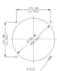
OUTLET SIDE
