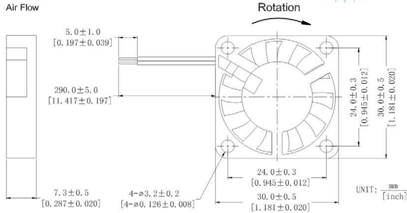
DIMENSIONS DRAWING
