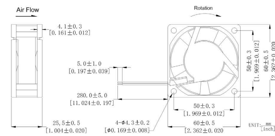
DIMENSIONS DRAWING
