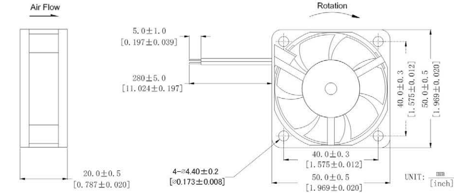
DIMENSIONS DRAWING
