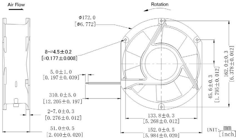
DIMENSIONS DRAWING
