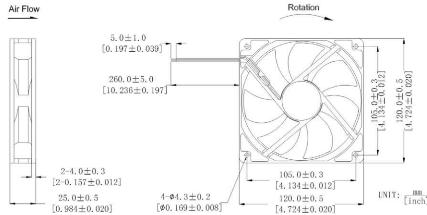
DIMENSIONS DRAWING
