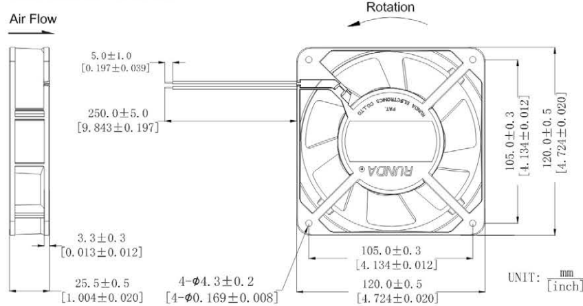
DIMENSIONS DRAWING
