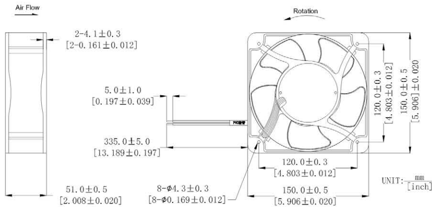
DIMENSIONS DRAWING
