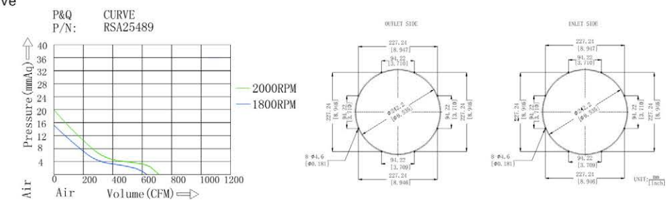
P&Q CURVE (AT RATED VOLTAGE)
