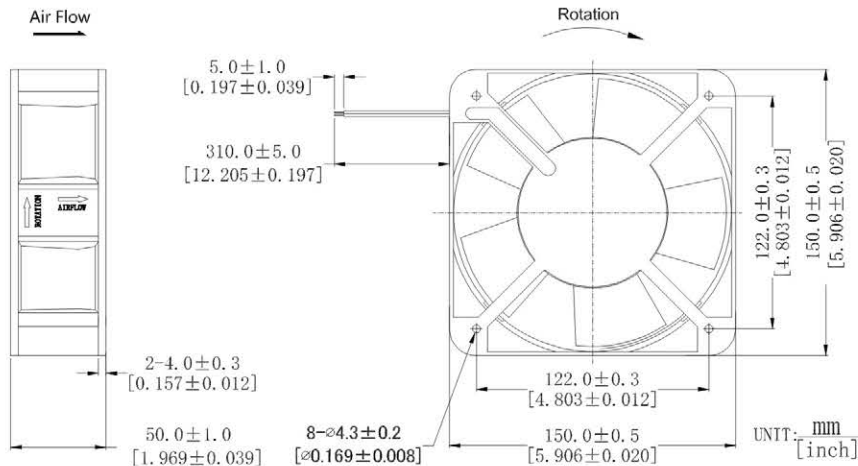
DIMENSIONS DRAWING
