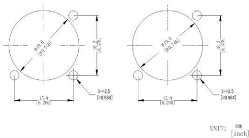
OUTLET SIDE
