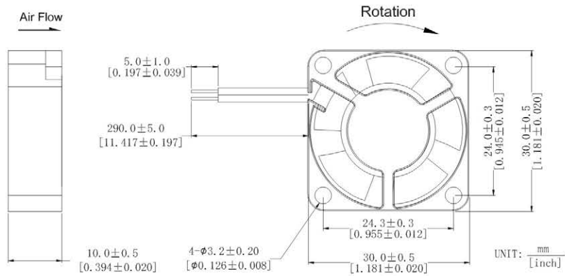
DIMENSIONS DRAWING
