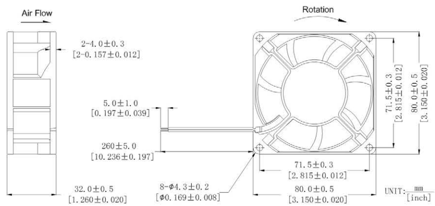
DIMENSIONS DRAWING
