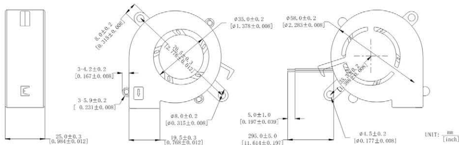
DIMENSIONS DRAWING
