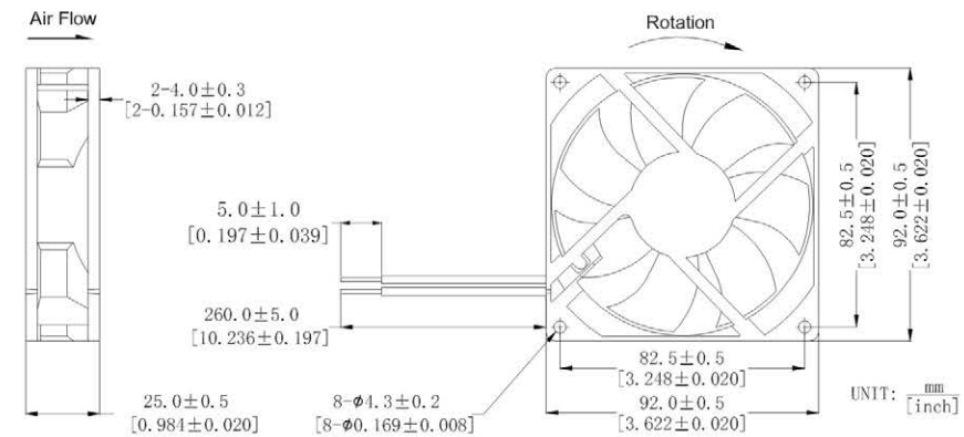
DIMENSIONS DRAWING
