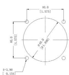
OUTLET SIDE
