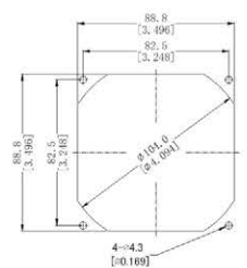
OUTLET SIDE
