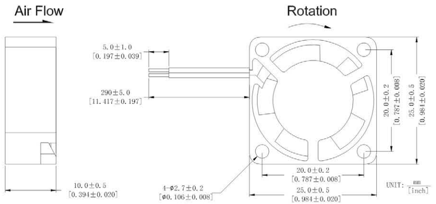
DIMENSIONS DRAWING
