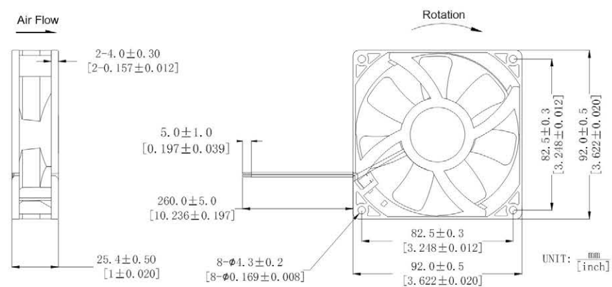
DIMENSIONS DRAWING
