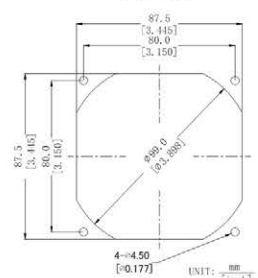
INLET SIDE
