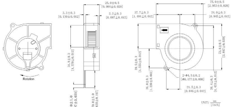
DIMENSIONS DRAWING
