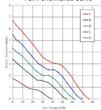
Fan Performance Curve
