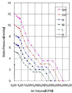
Fan Performance Curve
