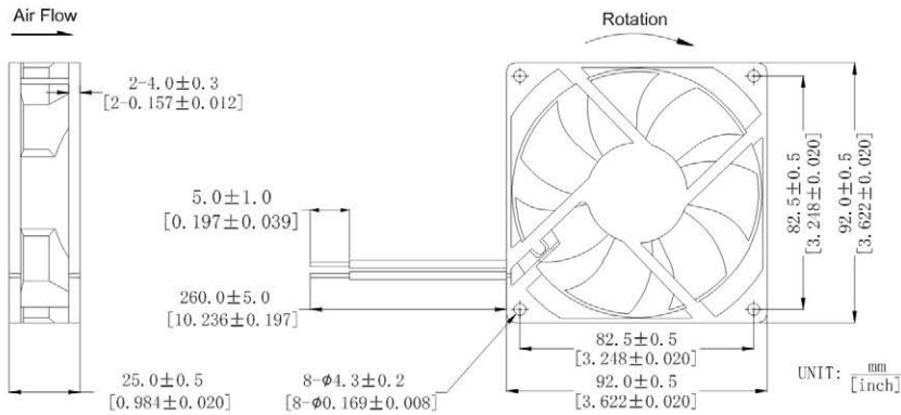
DIMENSIONS DRAWING
