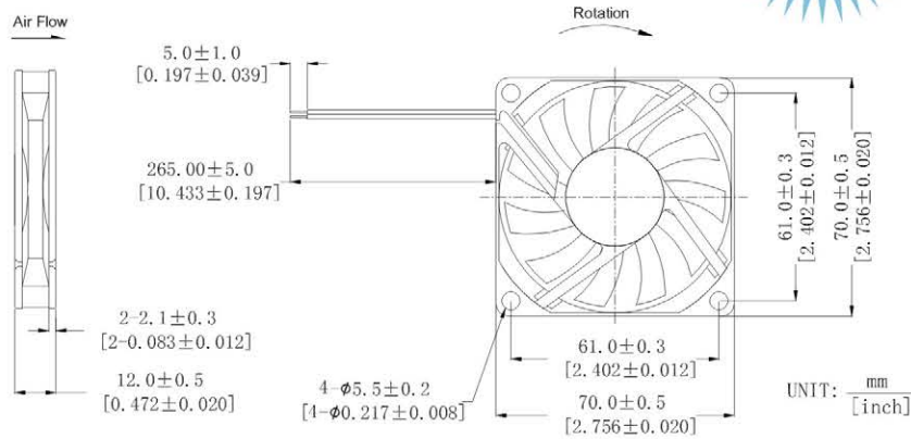
DIMENSIONS DRAWING
