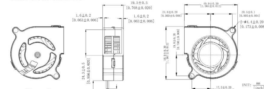
DIMENSIONS DRAWING
