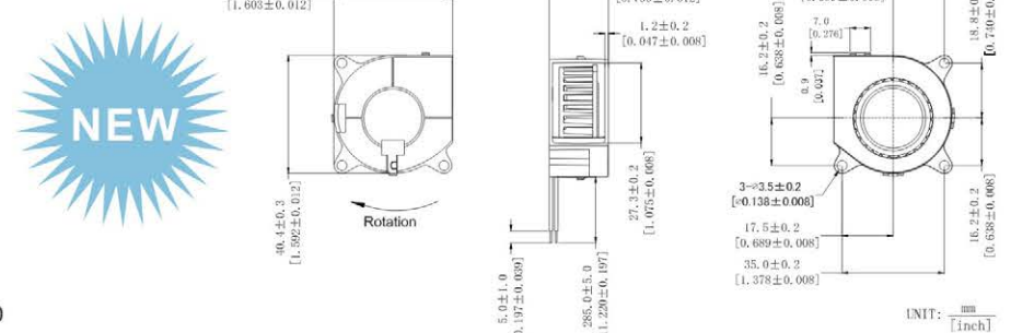
DIMENSIONS DRAWING
