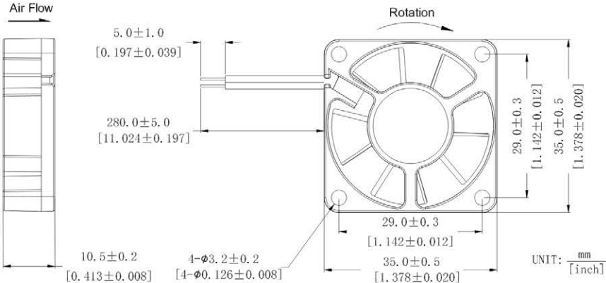
DIMENSIONS DRAWING
