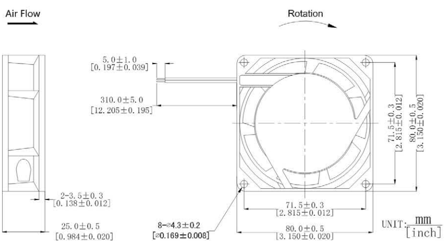
DIMENSIONS DRAWING
