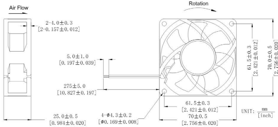
DIMENSIONS DRAWING
