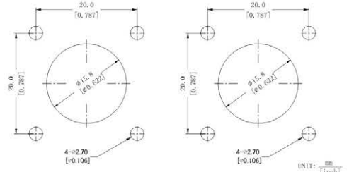
OUTLET SIDE
