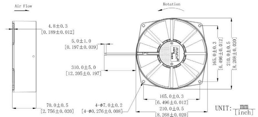
DIMENSIONS DRAWING
