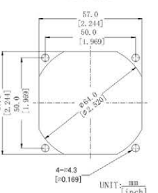
INLET SIDE
