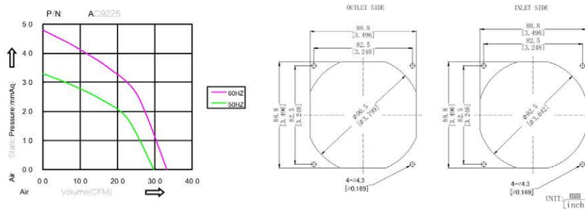
P&Q CURVE (AT RATED VOLTAGE)
