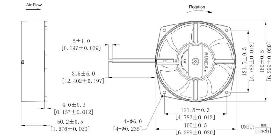
DIMENSIONS DRAWING
