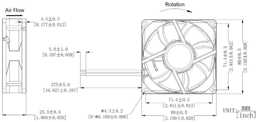
DIMENSIONS DRAWING
