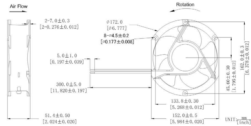
DIMENSIONS DRAWING
