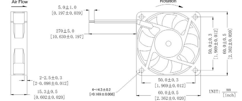
DIMENSIONS DRAWING
