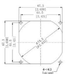
OUTLET SIDE
