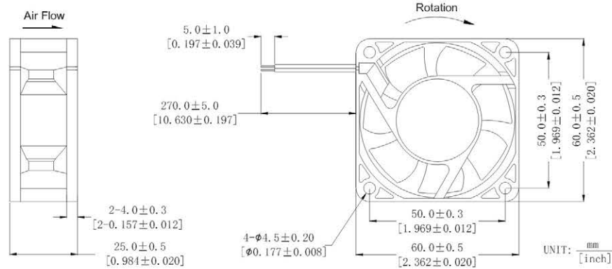
DIMENSIONS DRAWING
