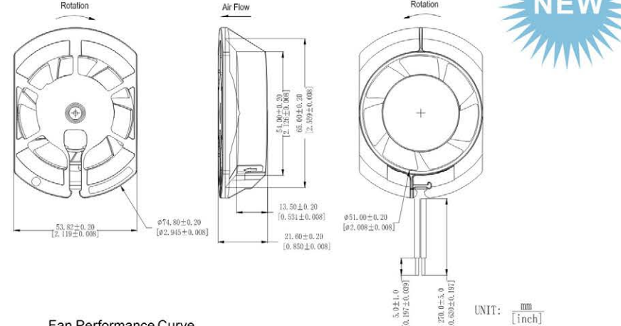
DIMENSIONS DRAWING
