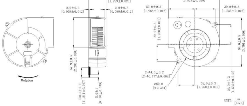
DIMENSIONS DRAWING
